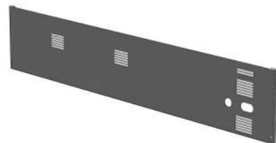
BACK TOP PANEL (REAR VIEW) 510-0719
