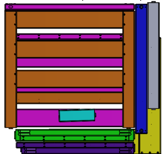
TOP VIEW (LESS SLING)
